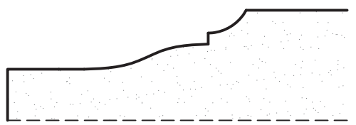
ROYAL PANEL (ROP)
