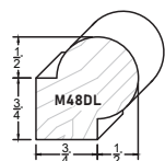
M48DL 1-1/4" x 1-1/4" 32mm x 32mm
