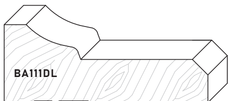
BA111DL 2" x 5-1/4" 51mm x 133mm
