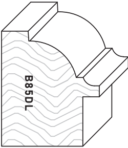
B85DL 1-1/2" x 1-3/4" 38mm x 44mm
