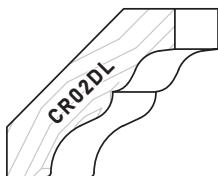
CR02DL Rise&Run=1-15/16" x 1-15/16" Size=3/4" x 2-3/4" 19mm x 70mm
