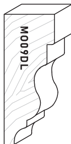
MO09DL 1\text{-}\frac{1}{4}'' \times 3\text{-}\frac{1}{4}'' 32mm x 83mm
