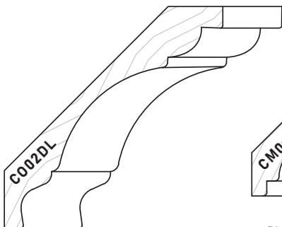
CO02DL* Rise&Run=3-11/16" x 3-11/16" Size=3/4" x 5-1/4" 19mm x 133mm
