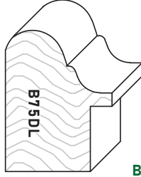
B75DL* 1-1/4" x 1-5/8" 32mm x 41mm
