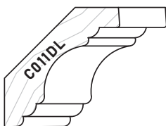
CO11DL Rise&Run=2" x 1-15/16" Size=3/4" x 2-3/4" 19mm x 70 mm
