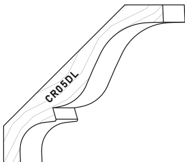
CR05DL* Rise&Run=3-11/16" x 3-11/16" Size=15/16" x 5-1/4" 23mm x 133mm
