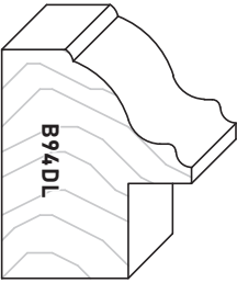
B94DL 1-1/2" \times 1-13/16" 38mm x 46mm
