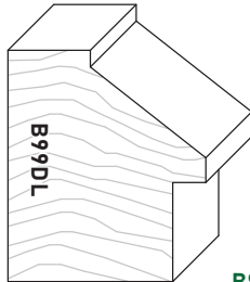
B99DL 1-1/2" \times 1-3/4" 38mm x 44mm
