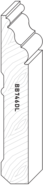
BB746DL 1-3/16" x 7-1/4" 30mm x 184mm Available: 9-1/4"=BB946DL (5-1/8")
