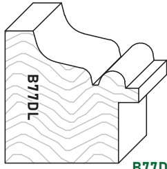
B77DL* 1-5/8" x 1-5/8" 41mm x 41mm
