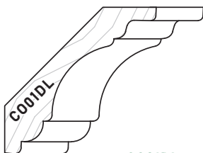
CO01DL Rise&Run=2-1/2" x 2-1/2" Size=3/4" x 3-1/2" 19mm x 89mm
