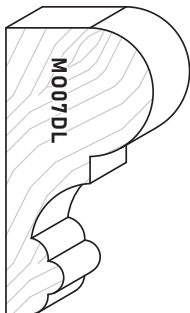
MO07DL 1\text{-}\frac{3}{4}'' \times 3\text{-}\frac{7}{16}'' 44mm x 87mm
