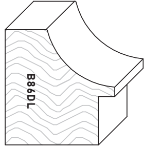
B86DL 1-11/16" x 1-13/16" 42mm x 46mm
