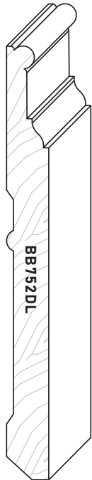
BB752DL 11/16" x 7-1/4" 17mm x 184mm Available: 4-1/4"=BB552DL 5-1/4"=BB552DL 9-1/4"=BB952DL (5-9/16")
