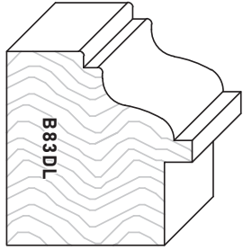
B83DL 1-11/16" x 1-3/4" 42mm x 44mm
