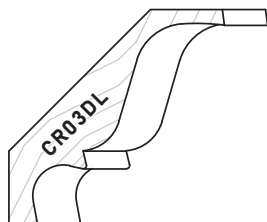
CR03DL* Rise&Run=2-1/2" x 2-1/2" Size=13/16" x 3-1/2" 21mm x 89mm
